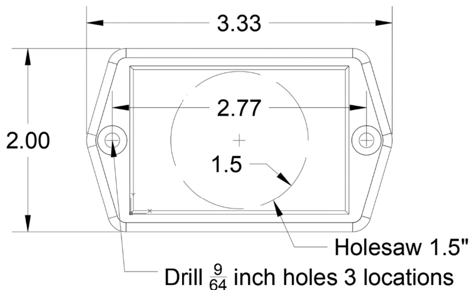
FIGURE 3.2 SPTSDL Outline Drawing
